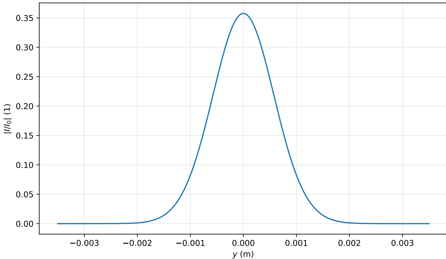
Intensity profile I(x=0, y, z=2.866)/I_0 , P_{in}=0.1P_{cr} , artificial time
